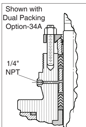
FIGURE 4 Leak-Off Conn. Option-26
